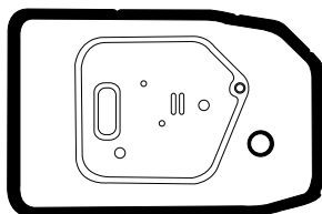
ZF5HP18 RWD - 5 Speed FK76800F
