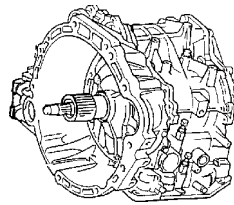
Underdrive (2 Piece Case)
